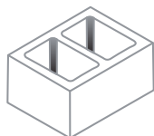
12" x 8" x 16" Regular
